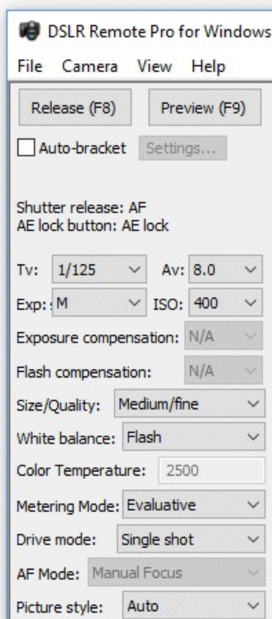
DSLR Remote Pro main window showing suggested camera settings for all camera models when using flash
